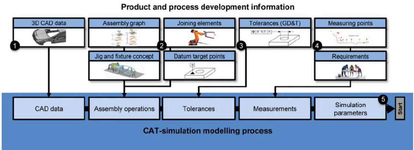
Figure 1: Dependencies of product and process information with regard to the CAT simulation model.
