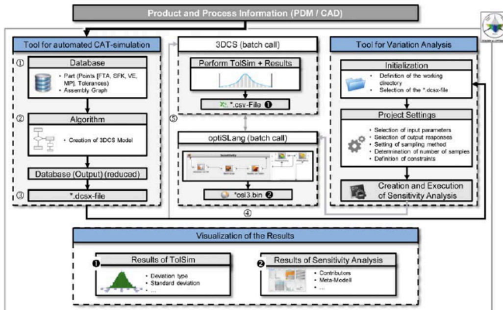
Figure 4: Implementation of the general approach in the automotive Body-in-White environment.
