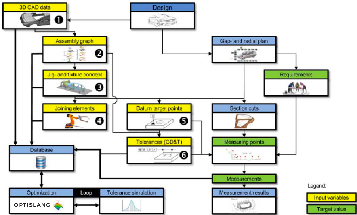
Figure 3: General approach for a sensitivity analysis of product and process information using tolerance simulations.
