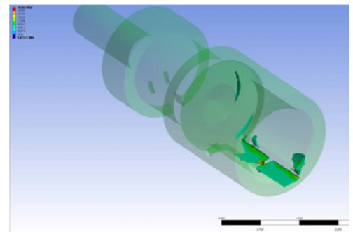
Part simulation of the rope pulley on the actuator unit, designed for infinite fatigue life.
