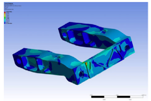
Assembly simulation of the prosthetic forefoot sides and crossbeam under maximum user loading against the dorsiflexion hard stop loading configuration.
