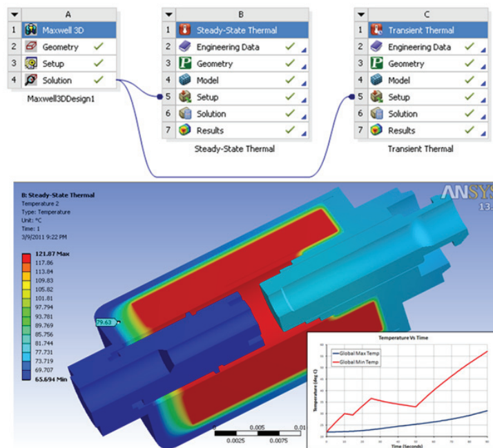
Figure 5: ANSYS Workbench enables mapping the losses from a magnetic simulation to a static and/or transient thermal simulation.
