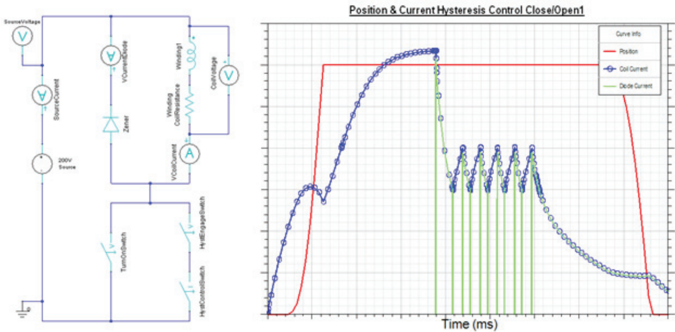
Figure 3: Using the circuit editor within Maxwell, a transient simulation with a chopped current controller is realized, showing transient waveforms of position, coil current and diode current.
