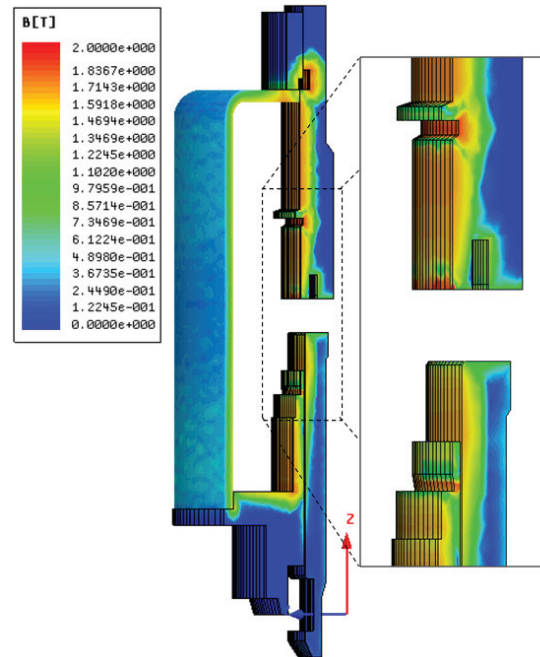
Figure 2: Magnetic flux density shown during a transient simulation after 0.001 seconds. Inset shows detail of the magnetic diffusion due to eddy currents. As time progresses, the fields diffuse through the thickness of the device, force increases, and the armature closes once the magnetic force overcomes spring and load forces.
