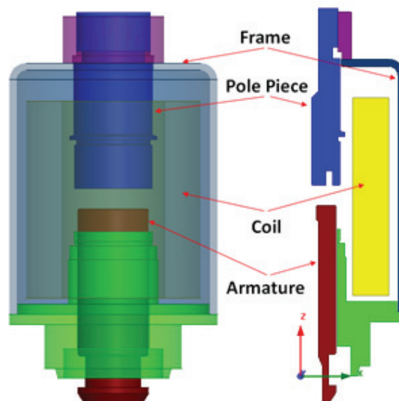
Figure 1: 3-D and axis-symmetric view of typical electromagnetic actuator, with frame, pole piece, coil and armature defined
