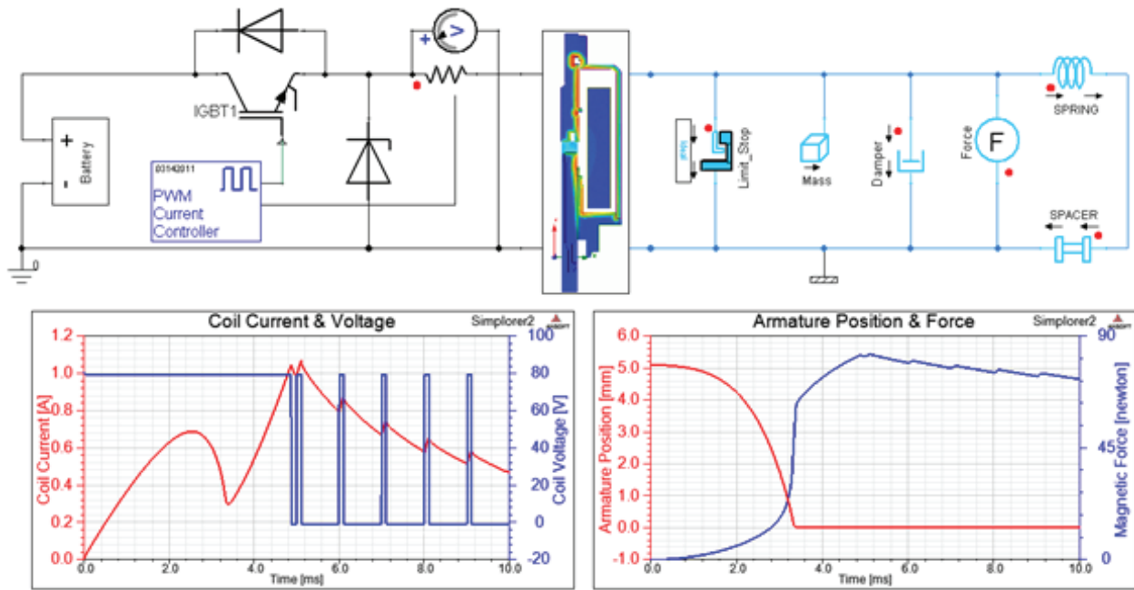
Figure 4: Robust system simulation in Simplorer showing a drive circuit coupled to the Maxwell FEA model through coupled transient link. Mechanical pins are connected to define mass, forces, springs and limit stops. Plots show coil current and voltage along with armature position and force versus time.
